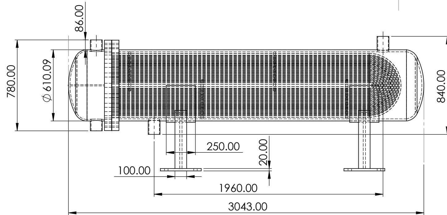
Front View
