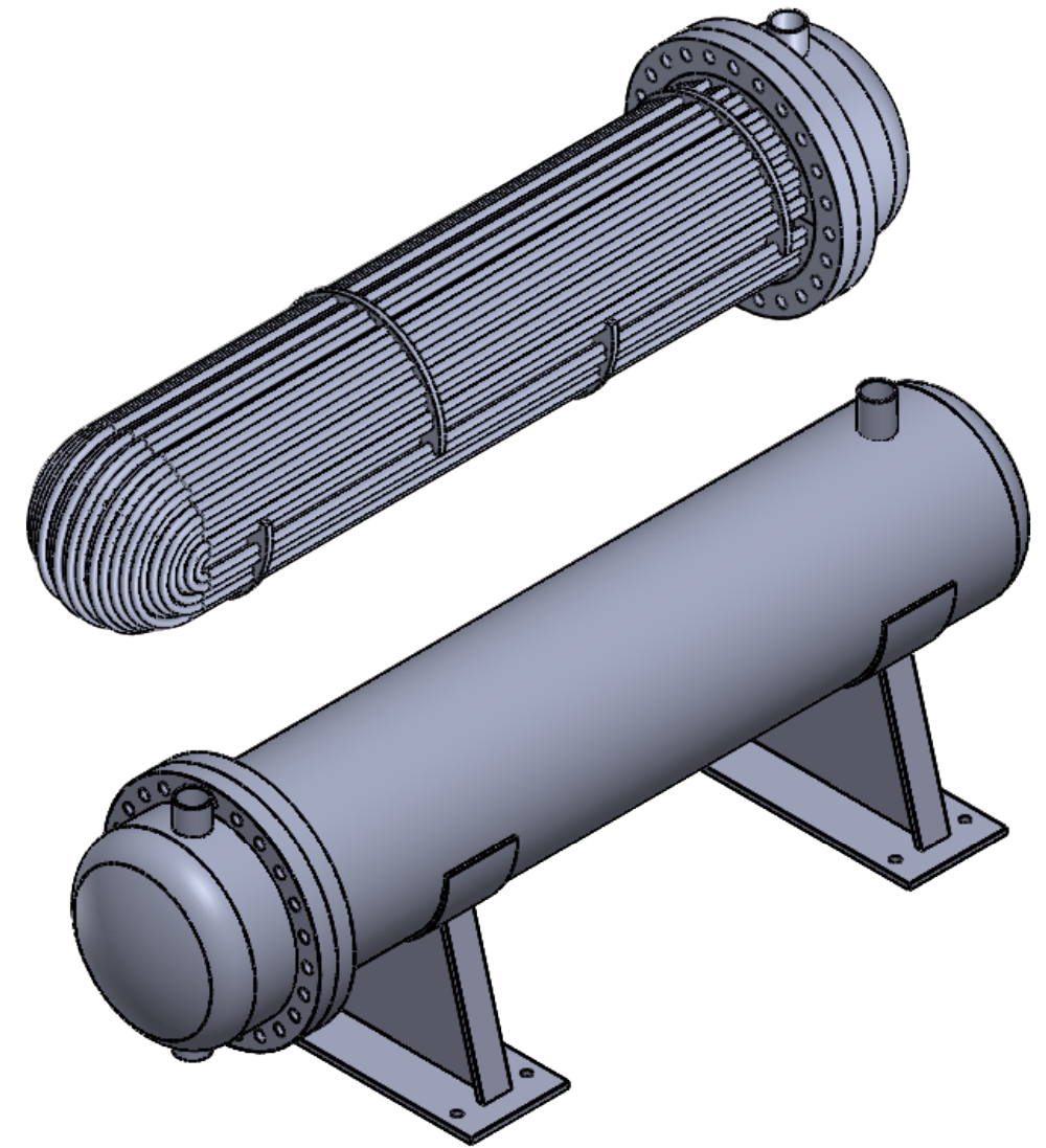
Isometric view
